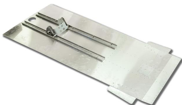
NAME: Floor panel, forward PART NO.: A32-01-005 WEIGHT: 1.8 kg
