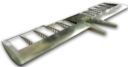
NAME: Stabilator, not covered PART NO.: A32-01-302 WEIGHT: 6.9 kg
