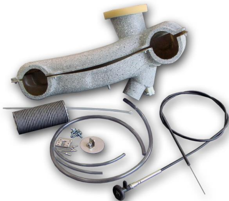
NAME: Intake airbox (a set) PART NO.: A32-03-150 WEIGHT: 0.7 kg
