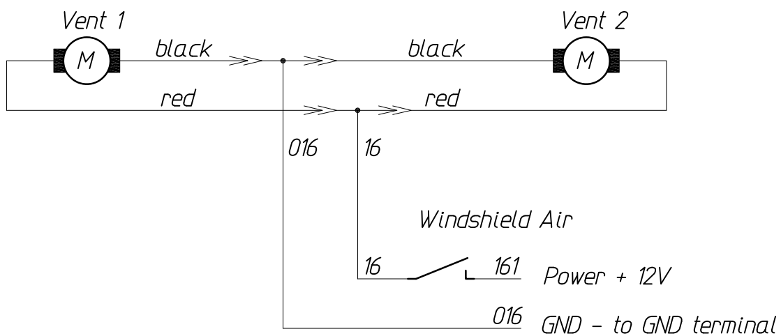
Fig. 22. Wiring diagram for installation of windshield air fans
