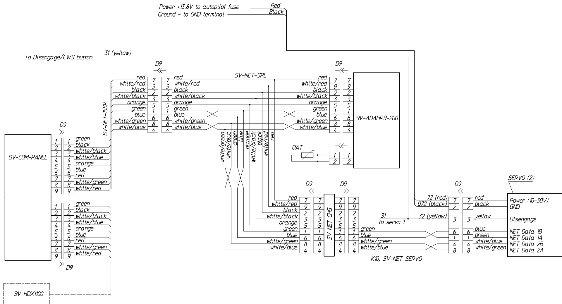
Fig. 18. Wiring diagram of Dynon SkyView system installation (page 3)
