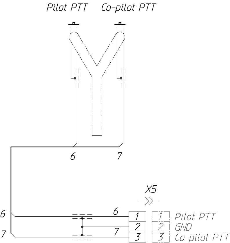
Fig. 23. Wiring diagram for installation of PTT buttons
