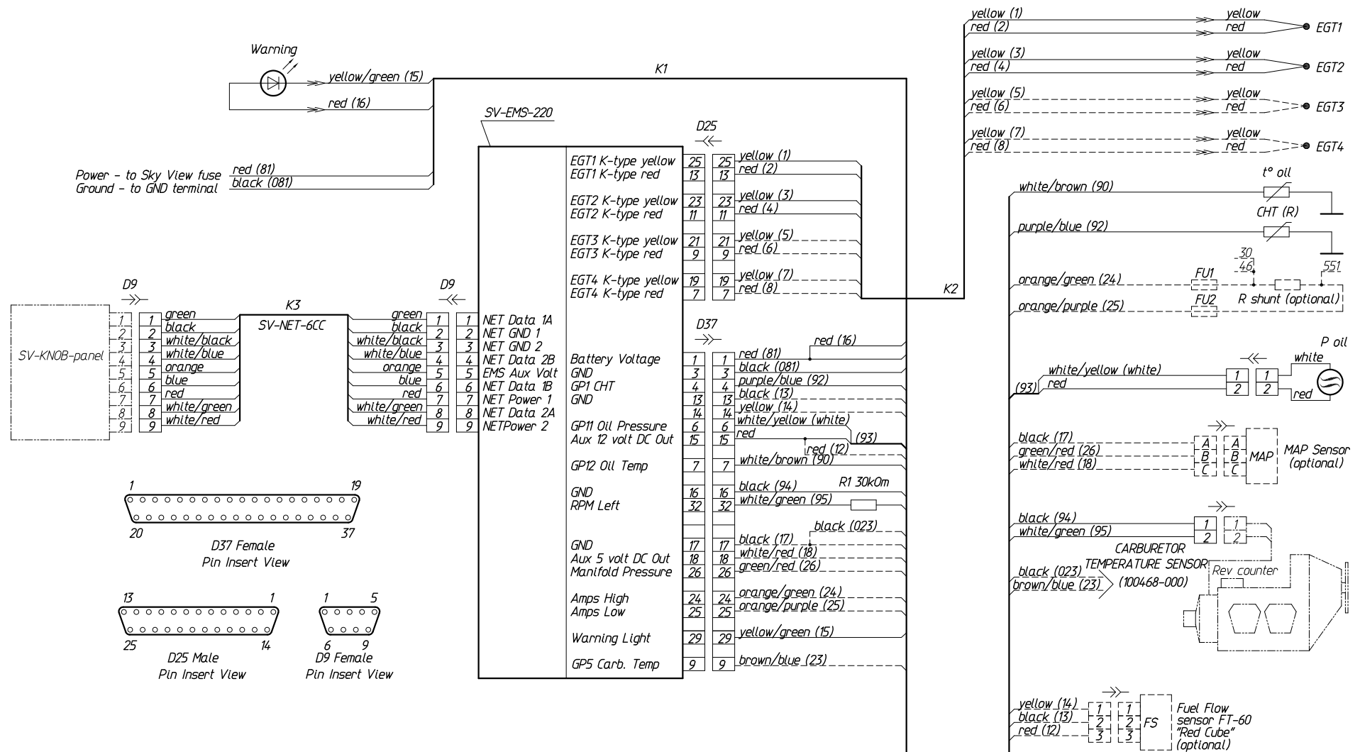
Fig. 16. Wiring diagram of Dynon SkyView system installation (page 1)
