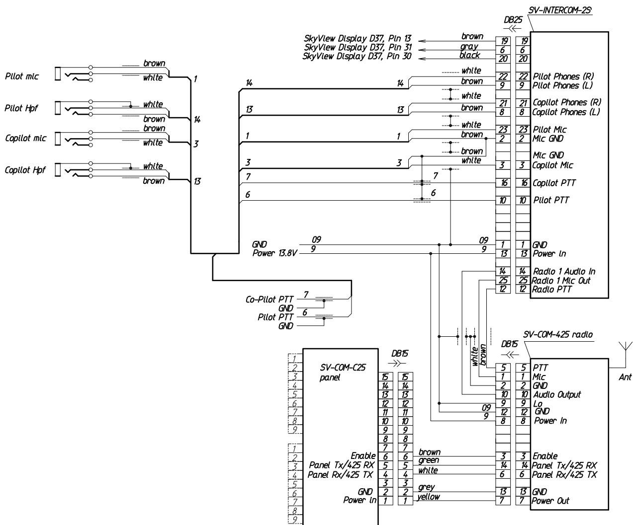
Fig. 20. Wiring diagram for installation of the Dynon SV-COM-425 radio
