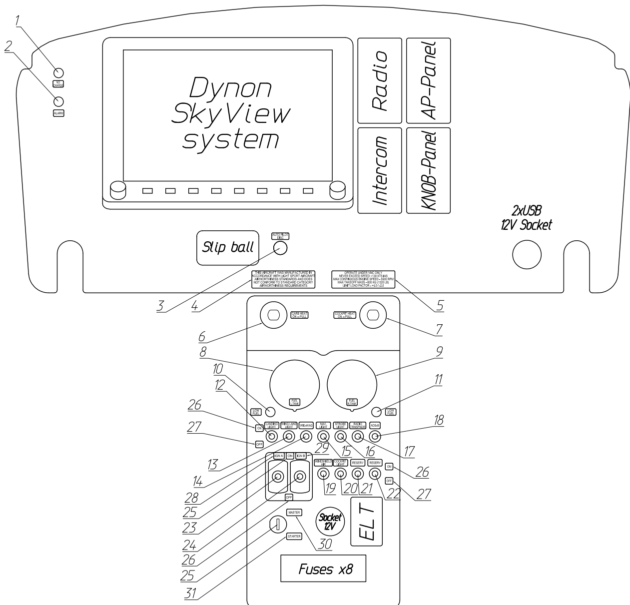
Fig. 13. Instrument panel
