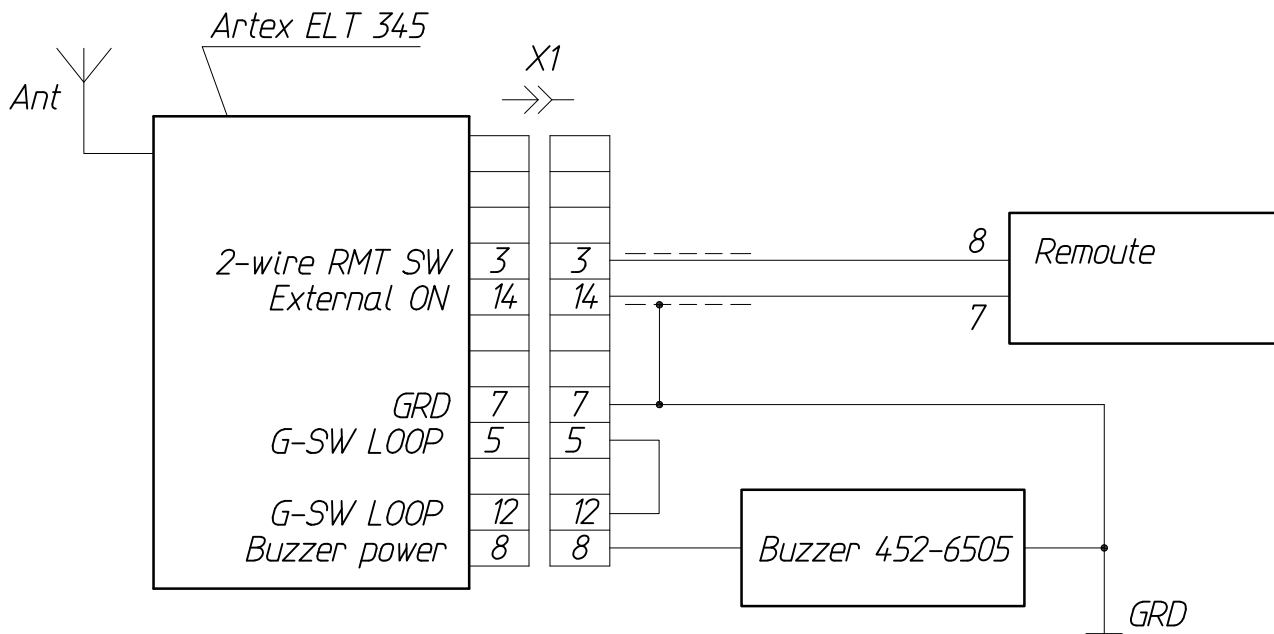
Fig. 19. Wiring diagram for installation of Artex ELT 345
